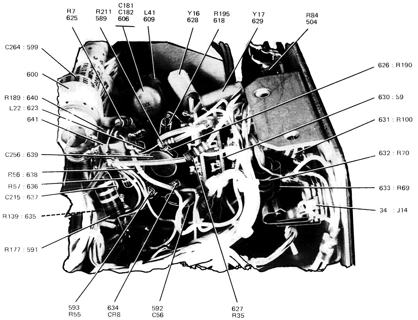
DETAIL P
