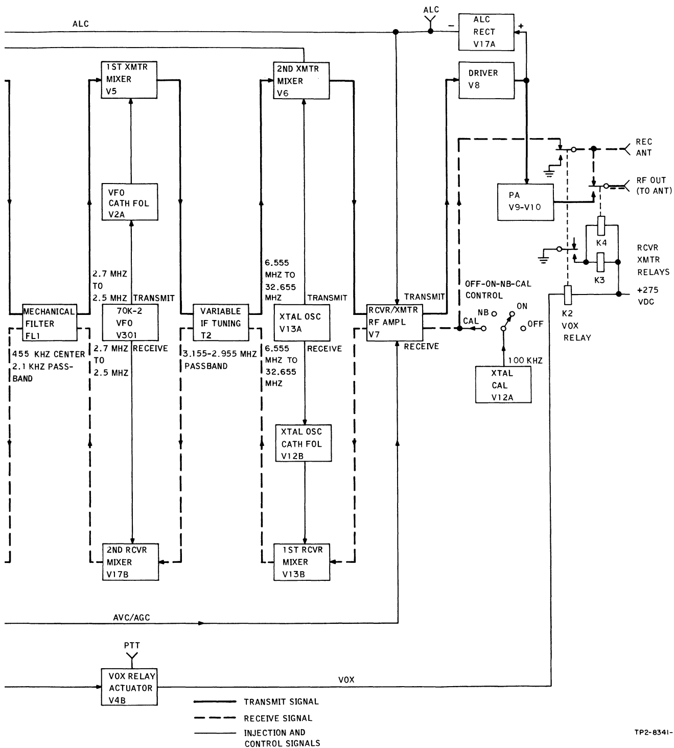
KWM-2 and KWM-2A Transceivers, Block Diagram Figure 3-1
